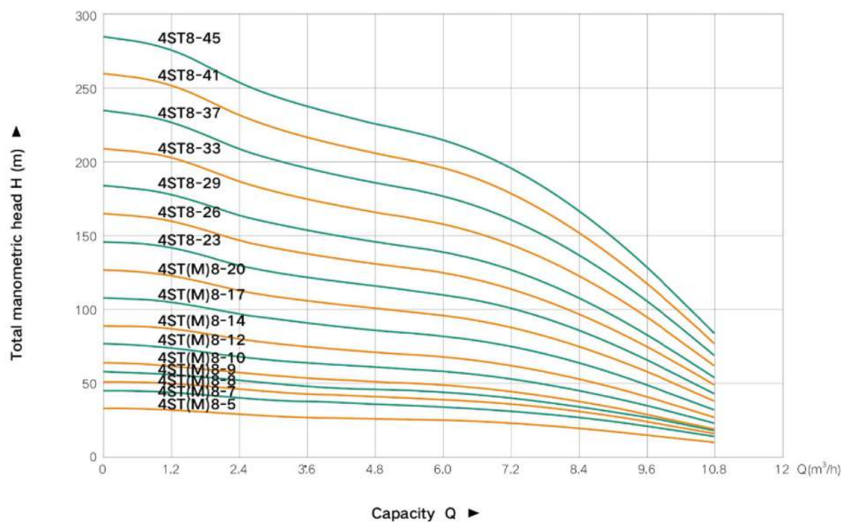
Performance Curve
