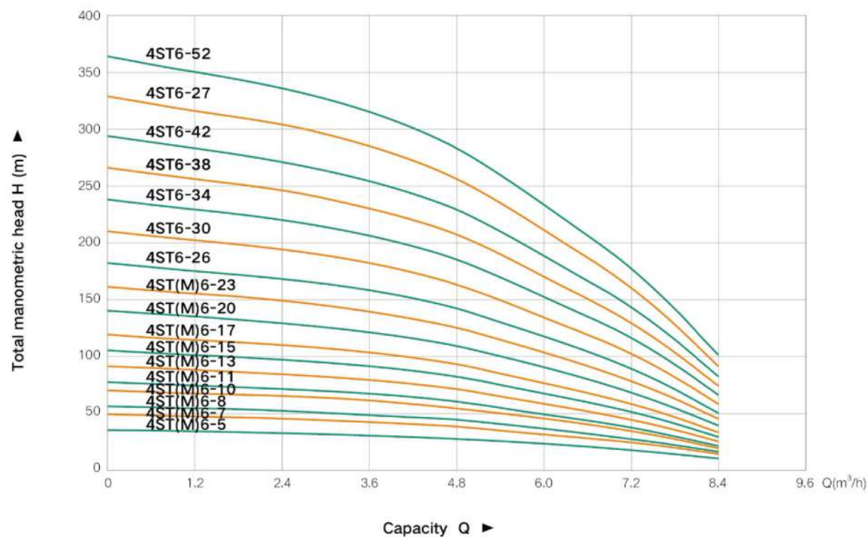
Performance Curve
